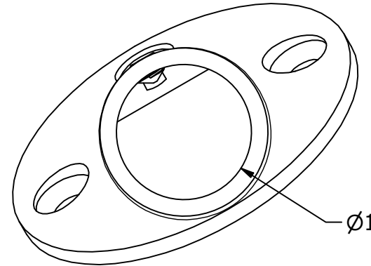
VIEW C-C SCALE 1 : 1
