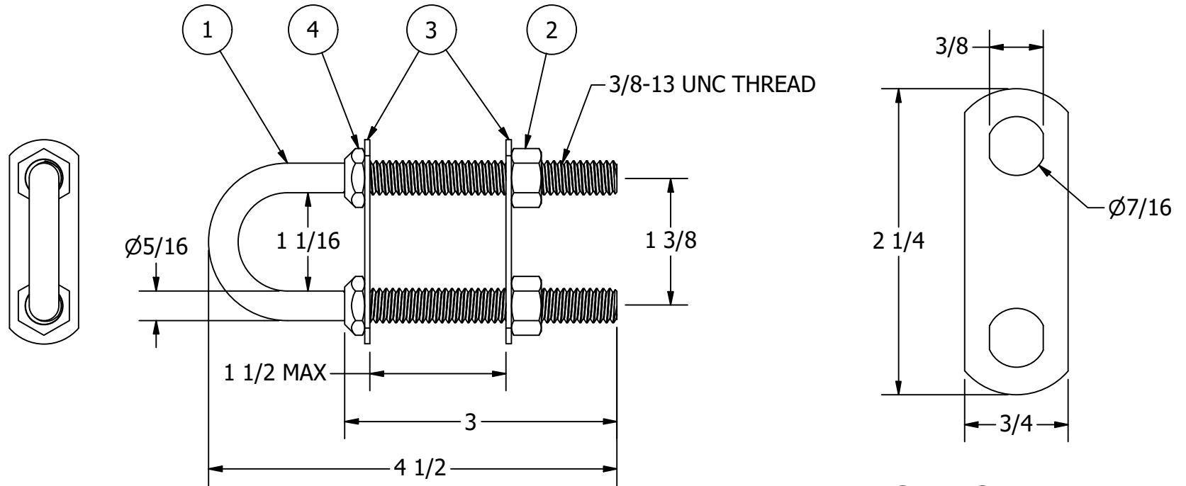
SUPPORT PLATE SCALE 1:1
