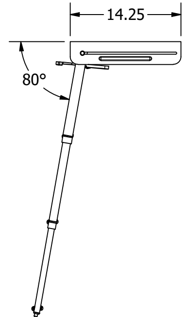
DEPLOYED VIEW SCALE 1 : 12
