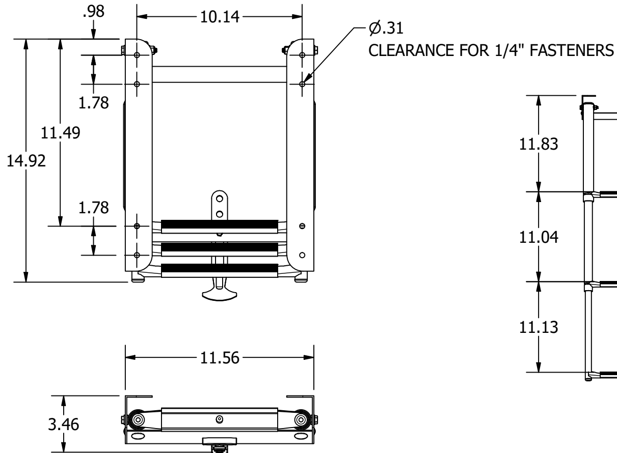
DEPLOYED VIEW SCALE 1 : 12
