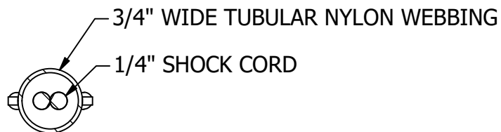
INTERNAL SECTION A-A SCALE 1 : 1
